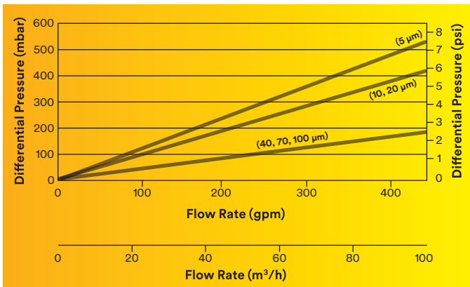
Graph 3. 60 Inch Cartridge
