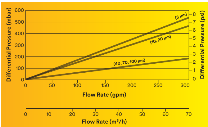
Graph 2. 40 Inch Cartridge
